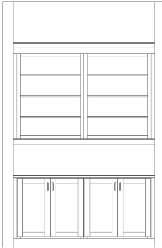
WALL A
